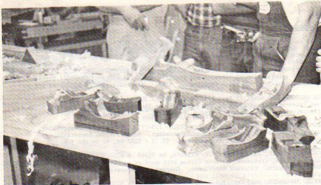
Some of the planes produced in the seminar, shown here almost finished near the end of the second day of the seminar.
